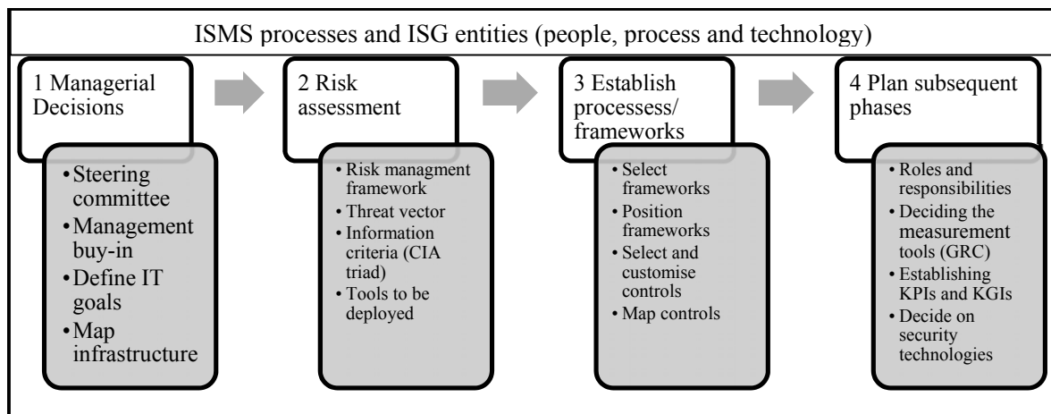
Figure 2. Plan stage of the ISG process
