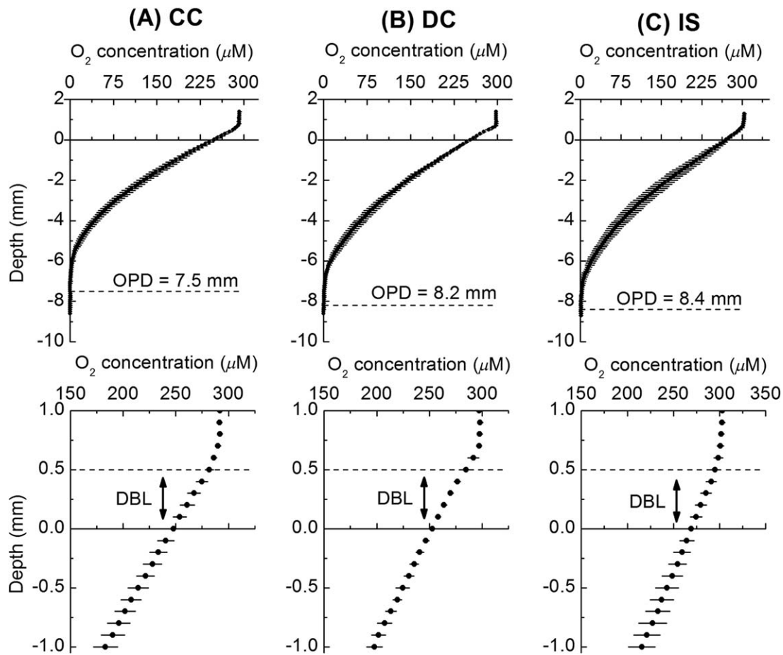
Fig. 2. Representative mean \pm SD oxygen microprofiles obtained from (A) Craib cores (CC, core 4, n=3 profiles), (B) SCUBA cores (DC, core 2, n=3 ) and (C) in situ lander (IS, n=10 ). X-axis indicates the sediment–water interface; oxygen penetration depth (OPD) is the depth in the sediment where the oxygen concentration first reaches zero. The bottom panels illustrate the approximate location and size of the diffusive boundary layer (DBL). DBL thickness was 300–600 \mu\text{m} .
