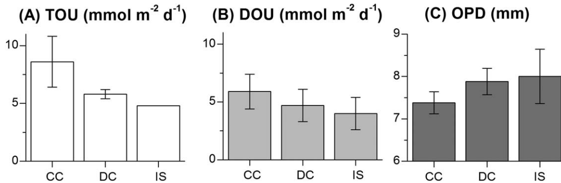
Fig. 3. (A) Total oxygen uptake (TOU, mean \pm SD; n = 5 for CC and DC, n = 1 for IS), (B) diffusive oxygen uptake (DOU, mean \pm SD; n = 15 for CC and DC, n = 10 for IS), and (C) oxygen penetration depth (OPD, mean \pm SD; n = 15 for CC and DC, n = 10 for IS) for the Craib cores (CC), SCUBA cores (DC) and the in situ lander (IS).
