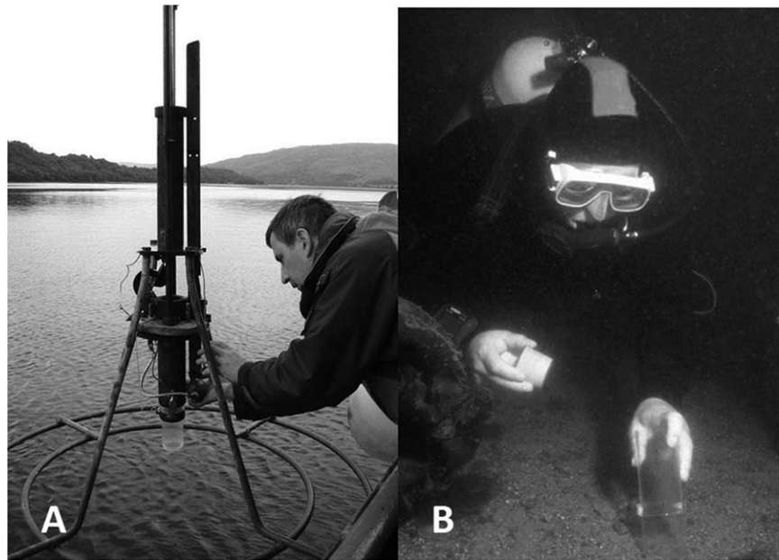
Fig. 1. (A) A Craib-corer being prepared for deployment; (B) A SCUBA diver manually coring sediments (note the bungs needed to seal the core tube).
