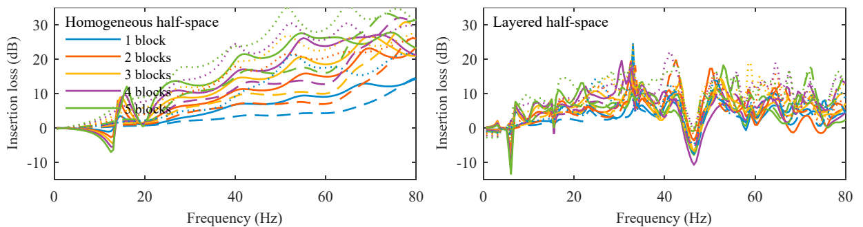
Fig. 4. Insertion loss as function of frequency for different numbers of blocks on a homogeneous half-space (left) or layered half-space (right). Full lines (—) indicate results for rigid solid blocks placed on top of the ground surface; dashed lines (---) indicate results for rigid solid blocks embedded 1.0 m into the ground; dotted lines (.....) indicate results for rigid solid blocks embedded 2.0 m into the ground.
