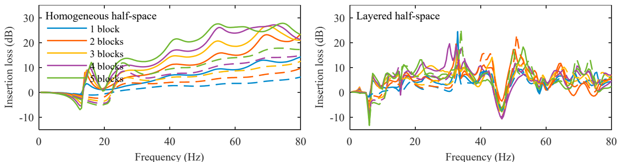
Fig. 3. Insertion loss as function of frequency for different numbers of blocks on a homogeneous half-space (left) or layered half-space (right). Full lines (—) indicate results for blocks with rotational inertia, whereas dashed lines (---) indicate results for blocks without rotational inertia.
