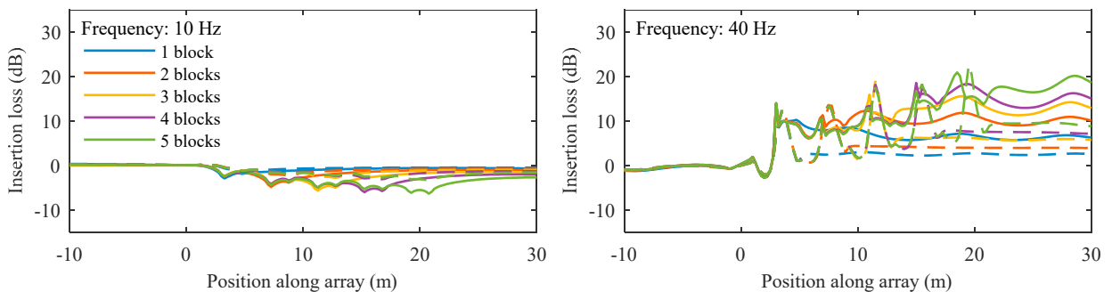
Fig. 2. Insertion loss as function of distance for different numbers of blocks on a homogeneous half-space at the frequencies 10 Hz and 40 Hz. Full lines (—) indicate results for blocks with rotational inertia, whereas dashed lines (---) indicate results for blocks without rotational inertia.
