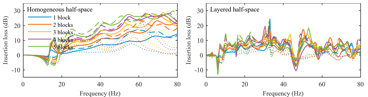
Fig. 5. Insertion loss as function of frequency for different numbers of blocks on a homogeneous half-space (left) or layered half-space (right). Full lines (—) indicate results for rigid solid blocks placed on top of the ground surface; dashed lines (---) indicate results for rigid plates embedded 1.0 m into the ground; dotted lines (.....) indicate results for rigid plates embedded 2.0 m into the ground.
