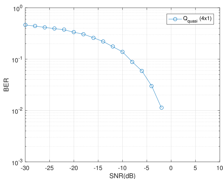
Figure 6. BER vs. SNR performance of Q_{quasi} for one receive dual-polarized antenna.
