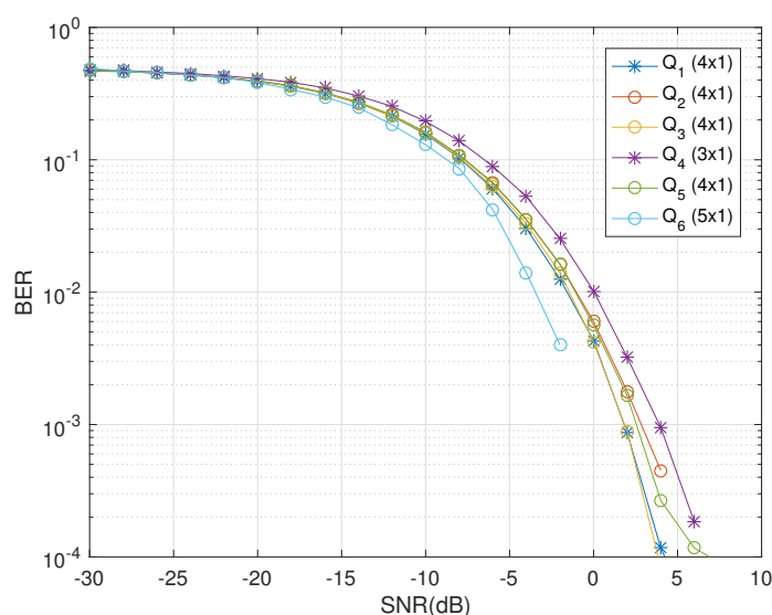
Figure 3. BER vs. SNR performance of Q_1, Q_2, Q_3, Q_4, Q_5 & Q_6 for single receive dual-polarized antenna.
