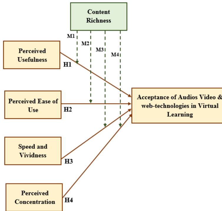
Fig. 1. Research model
