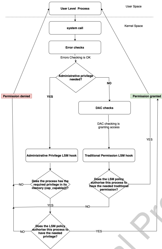
Figure 6. Current access control Decision algorithm implemented by Linux
