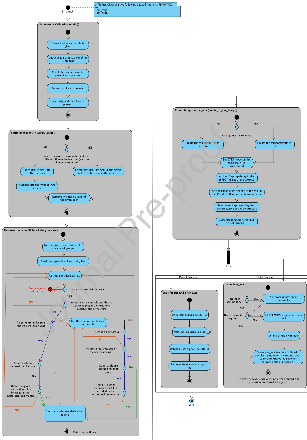
Figure 24. Flowchart for the sr command.
