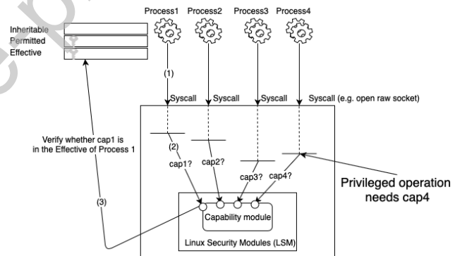
Figure 4. How capability's check works.
