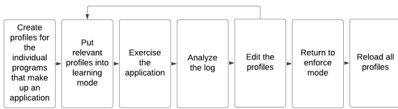
Figure 7. Systemic profiling method in AppArmor [26]
