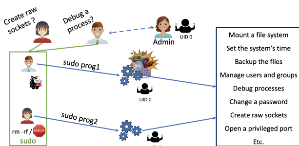
Figure 2. sudo command.
